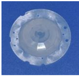
Model No.: 8604-5 Size: \varnothing 52.5*7.9 Focal length: 18mm Angel: 360 ° Distance: radius 7m ceiling mounting 2.5M
