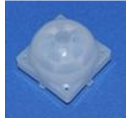
Model No.: 8002-1 (with hole) Size: 23.5*23.5*19 Focal length: 10.5mm Angel: 120° Distance: 10m
