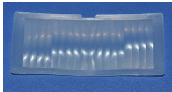
Model No.:7707-1A Size : 91.3*39.5 Focal length:25mm Angle:180 ° Distance:16m
