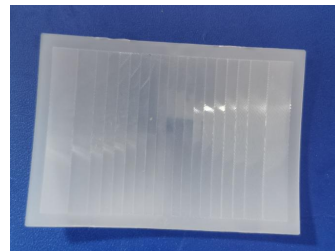
Model No.:YY-AA-V1 Size : 42.6*61 Focal length:30.5mm Angle:155 ° Distance:15m
