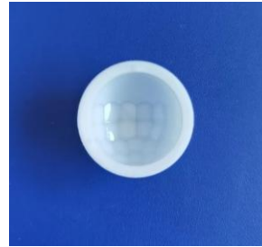
Model No.:YY-023115-15 Size: Ø26 Focal length: 11.5mm Angel: 120° Distance: DIA10m
