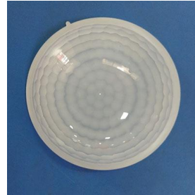
Model No.: YY-6725 Size: 69.6*71.3 Focal length: 20mm Angel: 360° Distance: Dia20m
