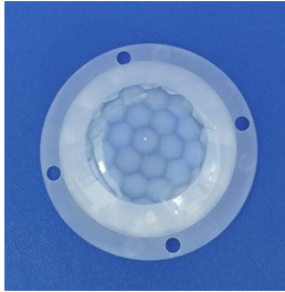
Model No.: 8605-3G Size: 44.5*12.2 Focal length: 15mm ceiling mounting 3M Angel: 360° Distance: Dia12m
