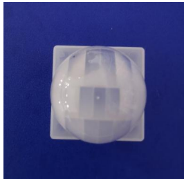
Model No.: YY-1003-45 Size: 24*24 Focal length: 12mm Angel: 120° Distance: 10m
