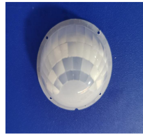
Model No.: YY-3518 Size: 39.83*18 Focal length: 17.5mm Angel: 160° Distance: 10m
