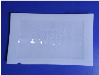
Model No.:YY-6531 Size : 63.3*51.15 Focal length:25mm Angle:120 ° Distance:≥ 10m
