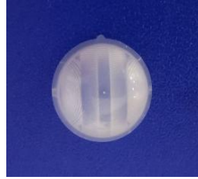
Model No.: YY-1102 Size: 14 Focal length: 6mm Angel: 130° Distance: 6m
