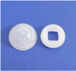
Model No.:13120-S19 Size: Ø14 Focal length: 6mm Angel: 120° Distance: 6m
