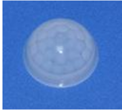
Model No.: 8003-2F Size: \varnothing 25.3*12.5 Focal length: 10.5mm Angel: 120 ° Distance: 12m
