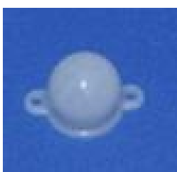
Model No.: 2136-1 Size: 23.8*16.3*13.1 Focal length: 7.5mm Angel: 120° Distance: 6m
