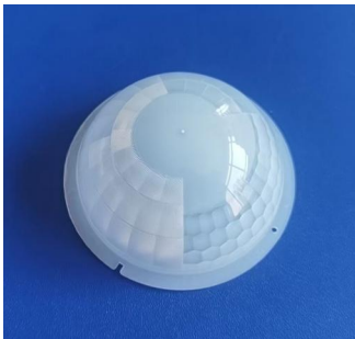
Model No.:YY-D52 Size: Ø52 Focal length: 17mm Angel: 240° Distance: 17m remarks: suitable for floodlights
