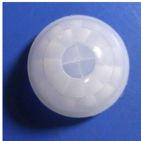
Model No.: X-23115-1 Size: 25.5 Focal length: 10.5mm Angel: 360° Distance: Dia10m
