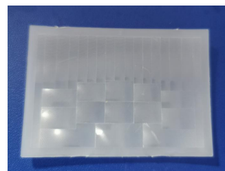
Model No.:YY-DWA-V2 Size : 42.6*61 Focal length:30.5mm Angle:101 ° Distance:9m
