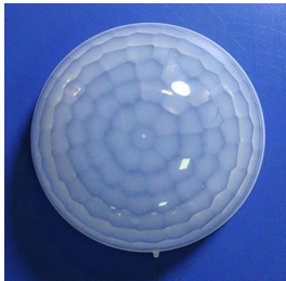
Model No.: YY-6030 Size: 63*64.49 Focal length: 29.8mm Angel: 360° Distance: Dia16m
