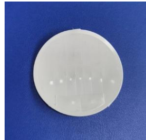
Model No.:GB-01-3640 Size : Ø40 Focal length:12mm Angle:90 ° Distance:12m-16m
