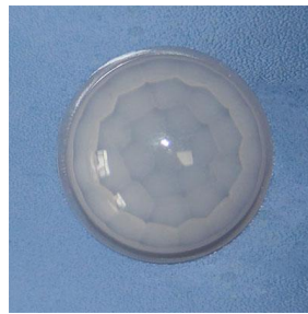
Model No.: 8003-2F-X Size: 25.5*12.3 Focal length: 10.5mm Angel: 120° Distance: 10m
