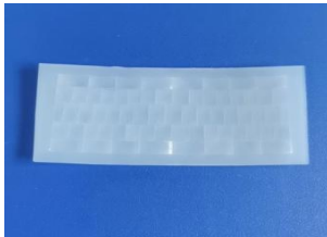
Model No.:8501-5 Size : 76*36.2 Focal length:20mm Angle:120 ° Distance:10m
