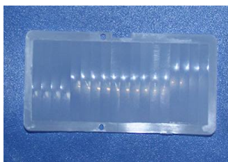
Model No.:7707-B Size : 39.5*85.3 Focal length:25mm Angle:180 ° Distance:16m
