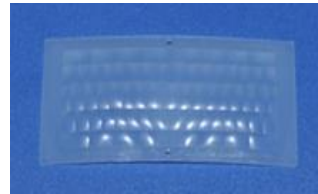
Model No.:614230 Size : 60.7*42.4 Focal length:30.5mm Angle:90 ° Distance:12m
