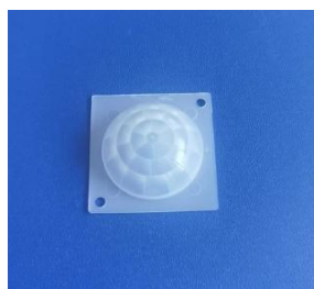
Model No.:HM-CM0.5-45 Size: Ø26.75 Focal length: 12.7mm Angel: 360° Distance: Dia18m
