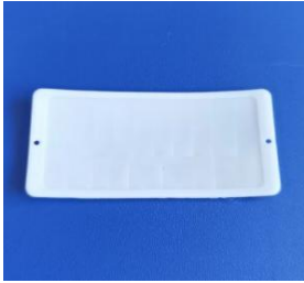
Model No.:WL-NK-04 Size : 54*25 Focal length:12mm Angle:120 ° Distance:8m
