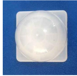
Model No.: 023100 (without legs) Size: 23.4*23.4*18.9 Focal length: 10.5mm Angel: 120° Distance: 10m
