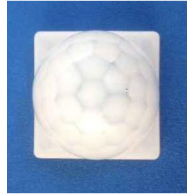
Model No.: 024120 (without legs) Size: 23.7*23.5*17.2 Focal length: 12mm Angel: 120° Distance: 12m
